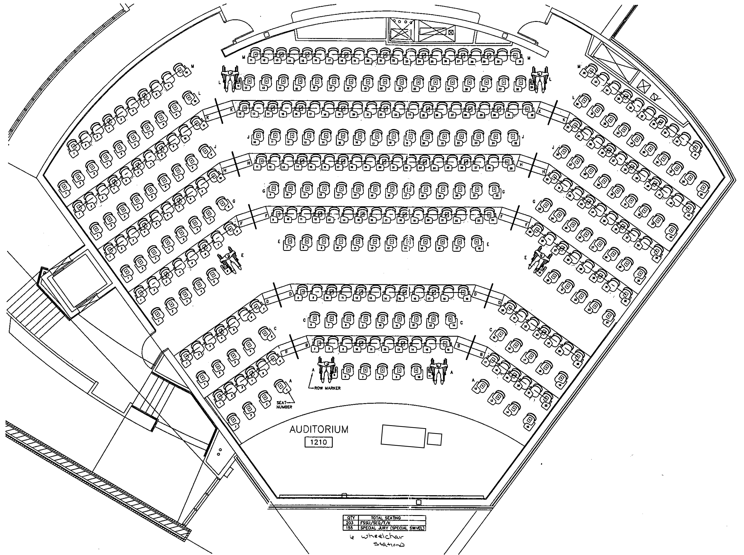
SEATING LAYOUT 3/8" = 1'-0"
